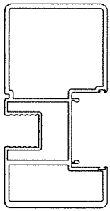
INTERLOCKS WITH REINF. ASTRAGAL W/O REINF.
