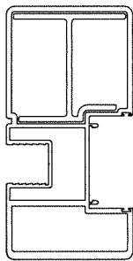
ASTRAGAL WITH REINF.
