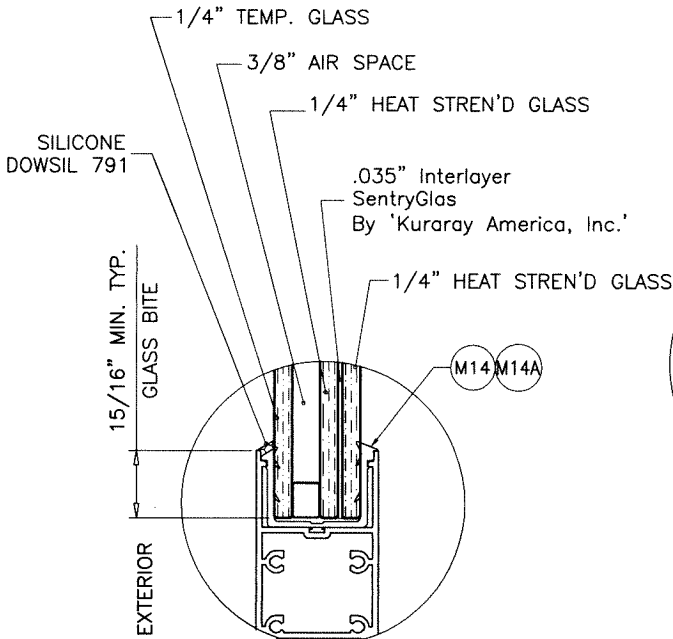
GLASS TYPE 'A2' 1-1/4" OVERALL INSUL. LAM. GLASS
