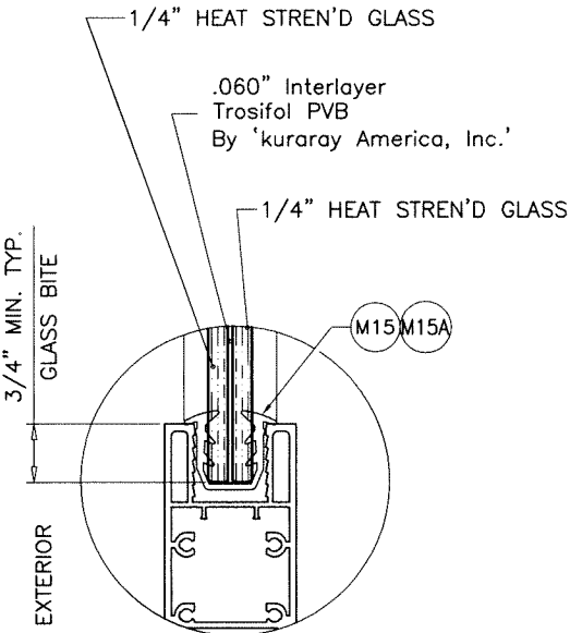
GLASS TYPE 'B' 9/16" OVERALL LAMINATED GLASS
