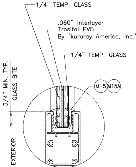
GLASS TYPE 'C' 9/16" OVERALL LAMINATED GLASS
