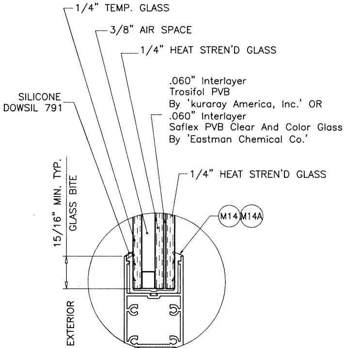
GLASS TYPE 'A1' 1-1/4" OVERALL INSUL. LAM. GLASS
