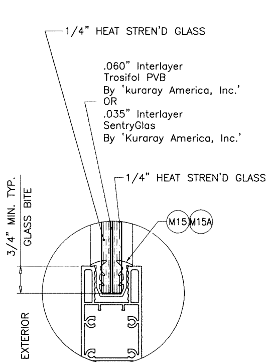
GLASS TYPE 'A' 9/16" OVERALL LAMINATED GLASS
