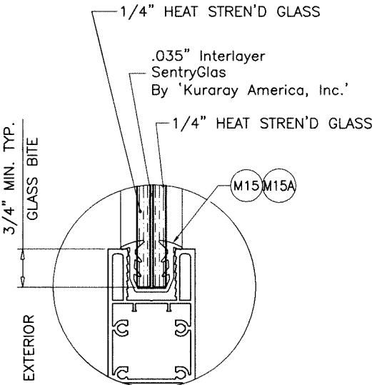
GLASS TYPE 'A.1' 9/16" OVERALL LAMINATED GLASS
