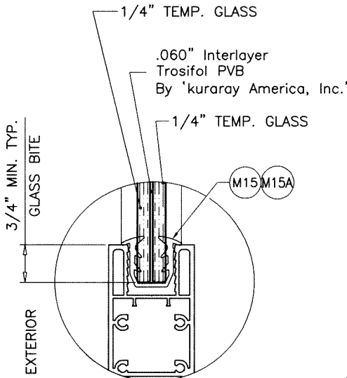
GLASS TYPE 'C' 9/16" OVERALL LAMINATED GLASS
